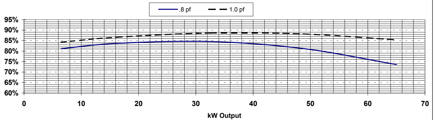
Efficiency at rated voltage and frequency vs. load kW
